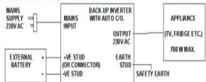
FIGURE 1 CONCEPT AND CONNECTION DIAGRAM.
