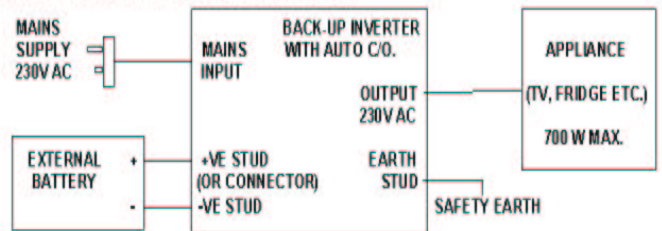
FIGURE 1 CONCEPT AND CONNECTION DIAGRAM.
